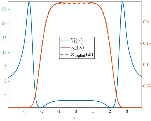
Fig. 3. Top hat potential V_l(x) that solves the inverse scattering problem in Eq. (27) with a top hat eigenfunction (26). The computed eigenfunction \varphi_d(x) is in solid red.
