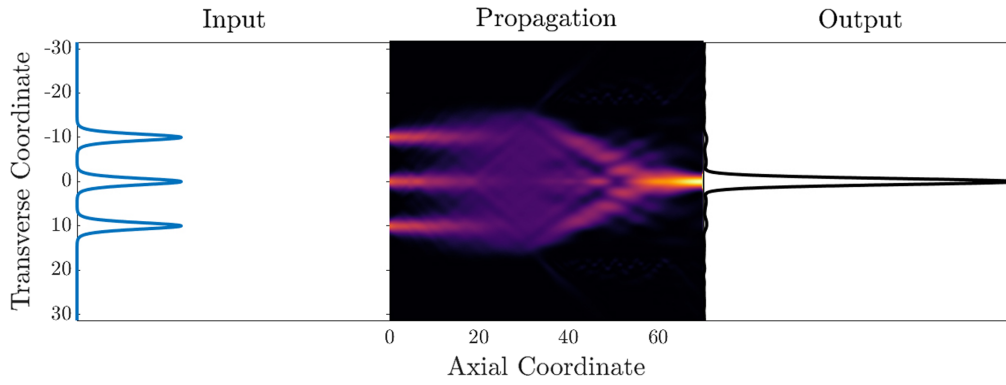
Fig. 1. Example of light reshaping in which three pulses of light are combined into one using the optimal control theory. More detail about the construction of the GRIN component, which combines these pulses, is provided throughout the paper.
