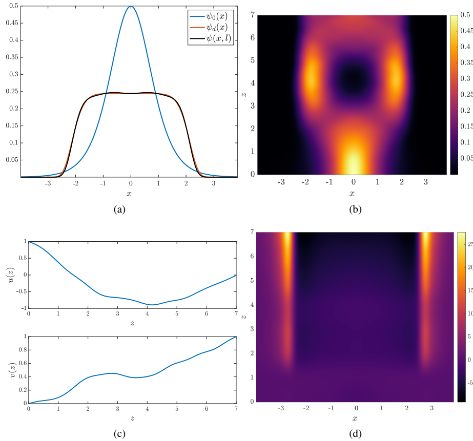
Fig. 4. Numerical solution of the top hat problem. (a) Intensity profiles for the initial, desired, and final computed wavefunctions. (b) Axial evolution of the wavefunction intensity. (c) Computed controls u(z) and v(z) resulting from the hybrid method. (d) Optimal potential resulting from (c) and the assumed form in Eq. (29).
