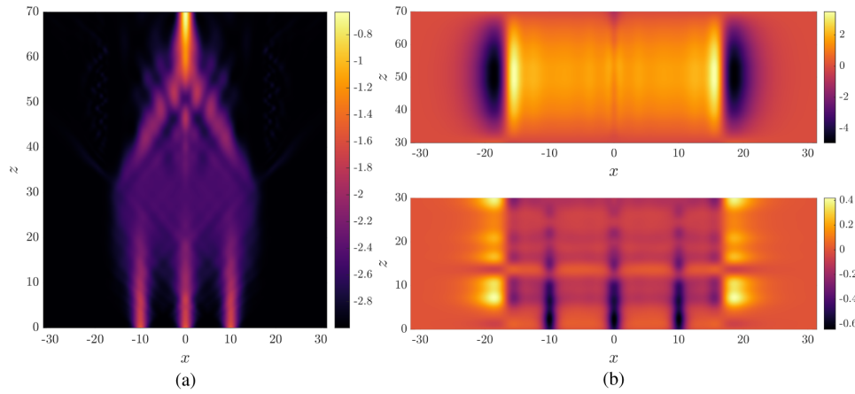
Fig. 5. (a) Schrödinger intensity distribution |\psi|^2 on a logarithmic scale. (b) Two stages of the computed optimal potential V(x, z) , shown separately because their ranges differ widely.
