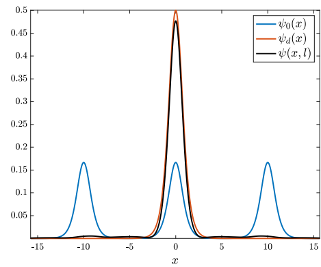
Fig. 6. Initial, desired, and final computed intensity profiles corresponding to Fig. 5.
