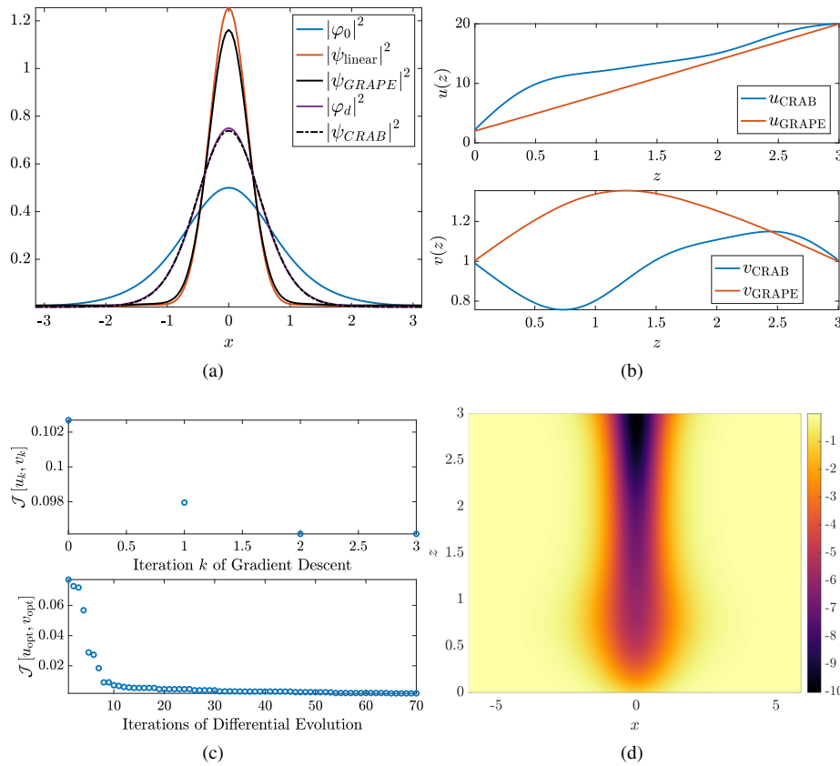
Fig. 2. Result of using the optimization methods in Sections 3.A and 3.B to reshape Pöschl–Teller eigenfunctions defined by Eq. (22). (a) Intensity profiles for the initial and desired eigenfunctions, a profile corresponding to linear controls, and profiles corresponding to the controls shown in (b), which are computed about linear controls via GRAPE and CRAB. (c) Local convergence of the descent method and the infidelity of optimal members from each iteration of differential evolution. (d) Potential V(x, u(z), v(z)) , cf. Eq. (21), resulting from the CRAB method.
